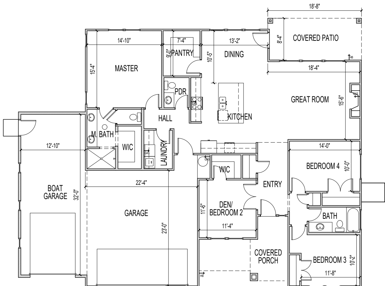
PLAN 1974G 1974 SQ.FT. 68'-4"x53'-8"
