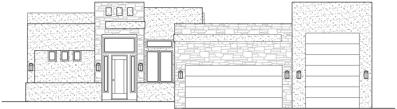
PLAN 2282F 2282 SQ.FT. 64'-0"x65'-0"
