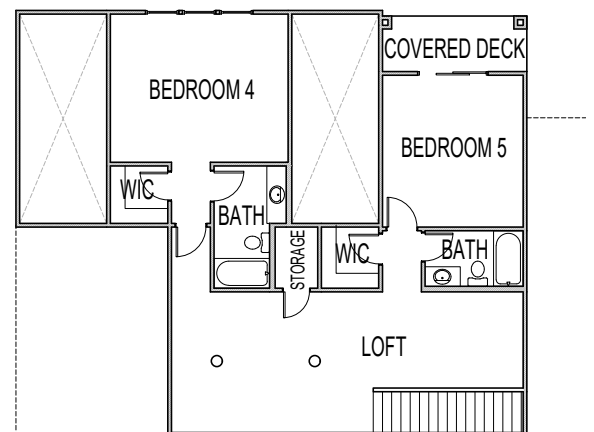
UPPER FLOOR
