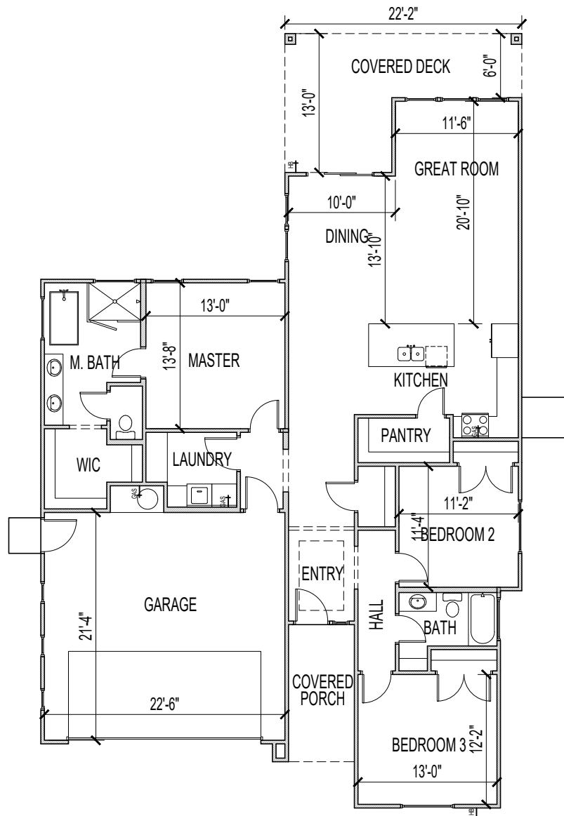
PLAN 1738G 1738 SQ.FT. 45'-0"x72'-6"
