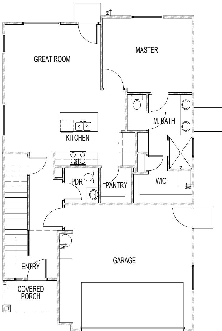
MAIN FLOOR
