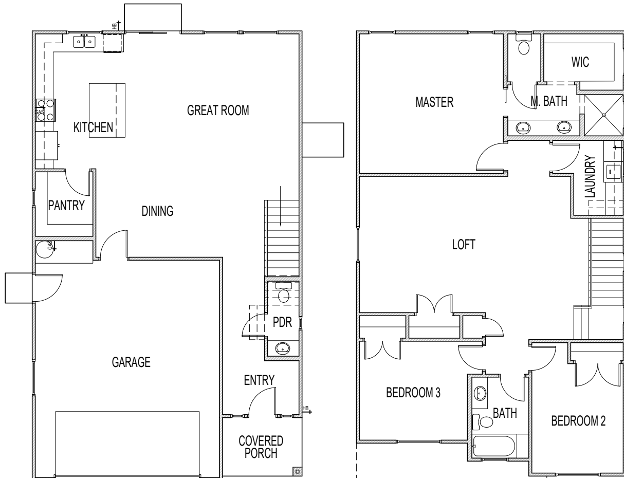
PLAN 2339G 2339 SQ.FT. 30'-0"x50'-0"
