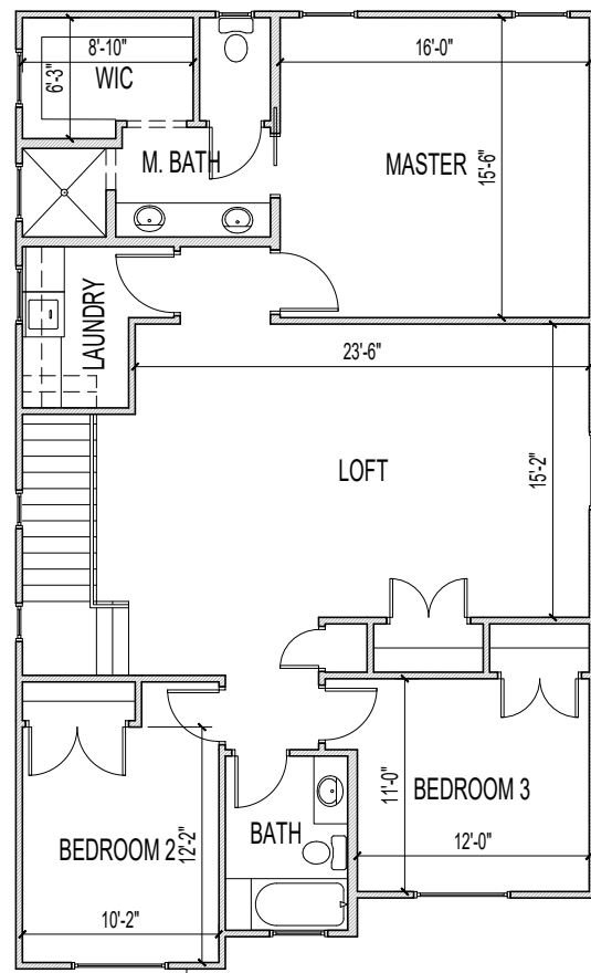
PLAN 2339G 2339 SQ.FT. 30'-0"x50'-0"
