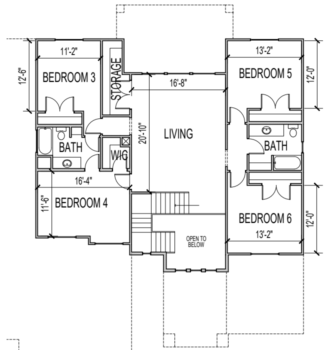
UPPER FLOOR
