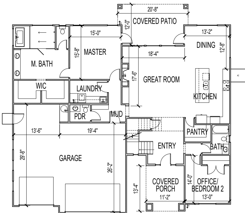
MAIN FLOOR
